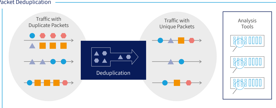
Packet Deduplication
