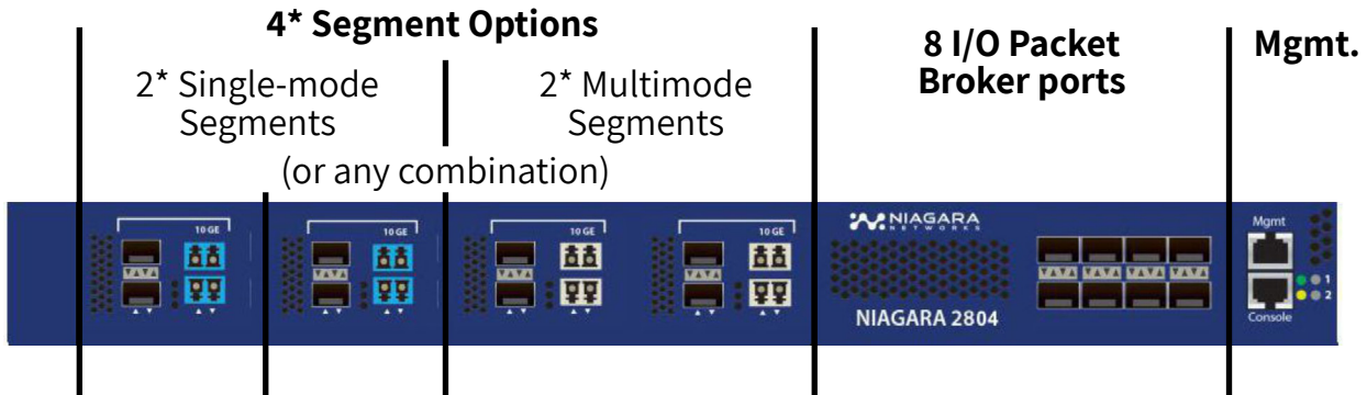
Figure 9: 2804 front panel depicting four segments, and eight additional I/O packet broker ports
