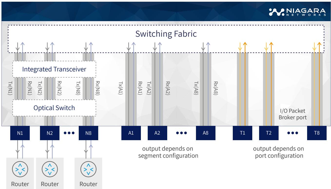
Figure 10: Integrated additional 8 I/O packet broker ports
